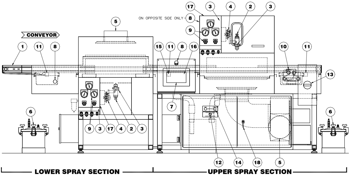
Figure: Major Components of the 9524D Spray System with right-hand controls
