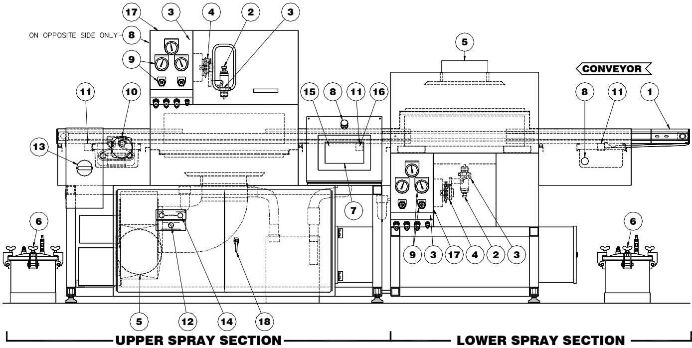
Figure: Major Components of the 9524D Spray System with left-hand controls
